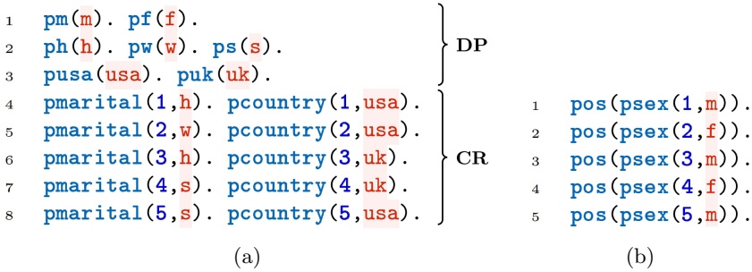
Fig. 1. Encoding the dataset from Table 1 in Popper: (a) background knowledge: decision points ( DP ) and column relations ( CR ), and (b) examples.
